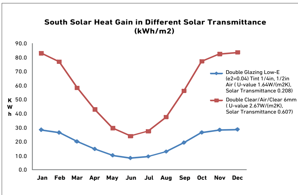
Figure 7 South Solar Heat Gain in Different Solar Transmittance (kWh/m 2 )
