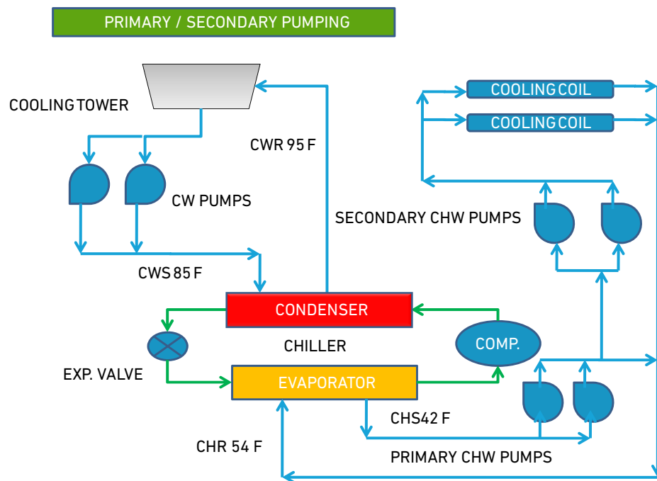
Figure 14 Primary/Secondary Pumping
